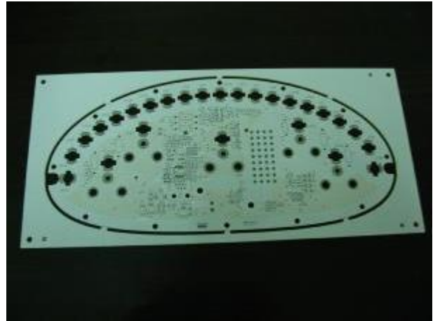
Beyaz / White PCB
